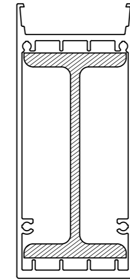
CR220 + VR063 I_{xx} = 773.3685 \text{ cm}^4
