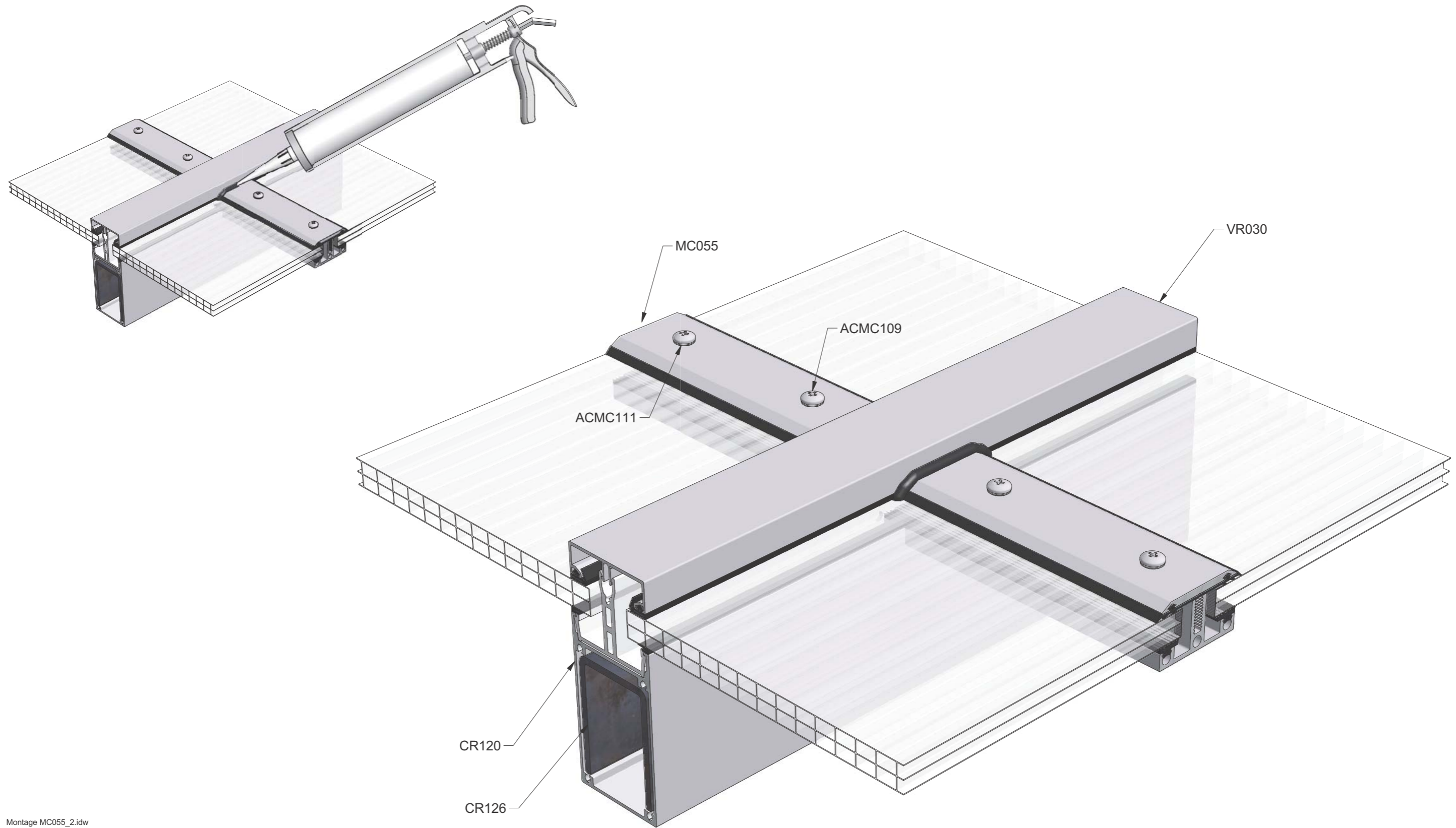
Montage MC055_2.idw
