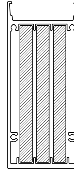
CR220 + 3x staal 110x10 mm I_{xx} = 1249.0335 \text{ cm}^4
