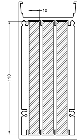
CR220 + 3x staal 110x10 mm I_{xx} = 1249.0335 \text{ cm}^4
