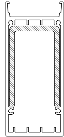
CR220 + CR226 I_{xx} = 446.1195 \text{ cm}^4
