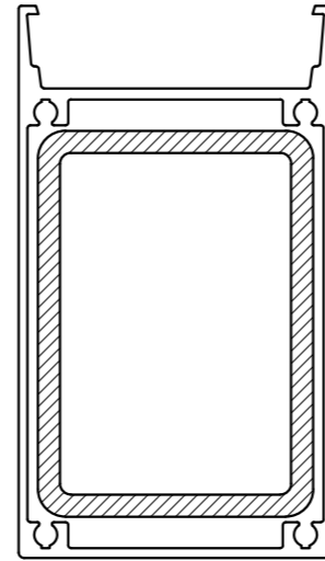
CR120 + Staal 70x50x4 mm I_{xx} = 251.5789 \text{ cm}^4
